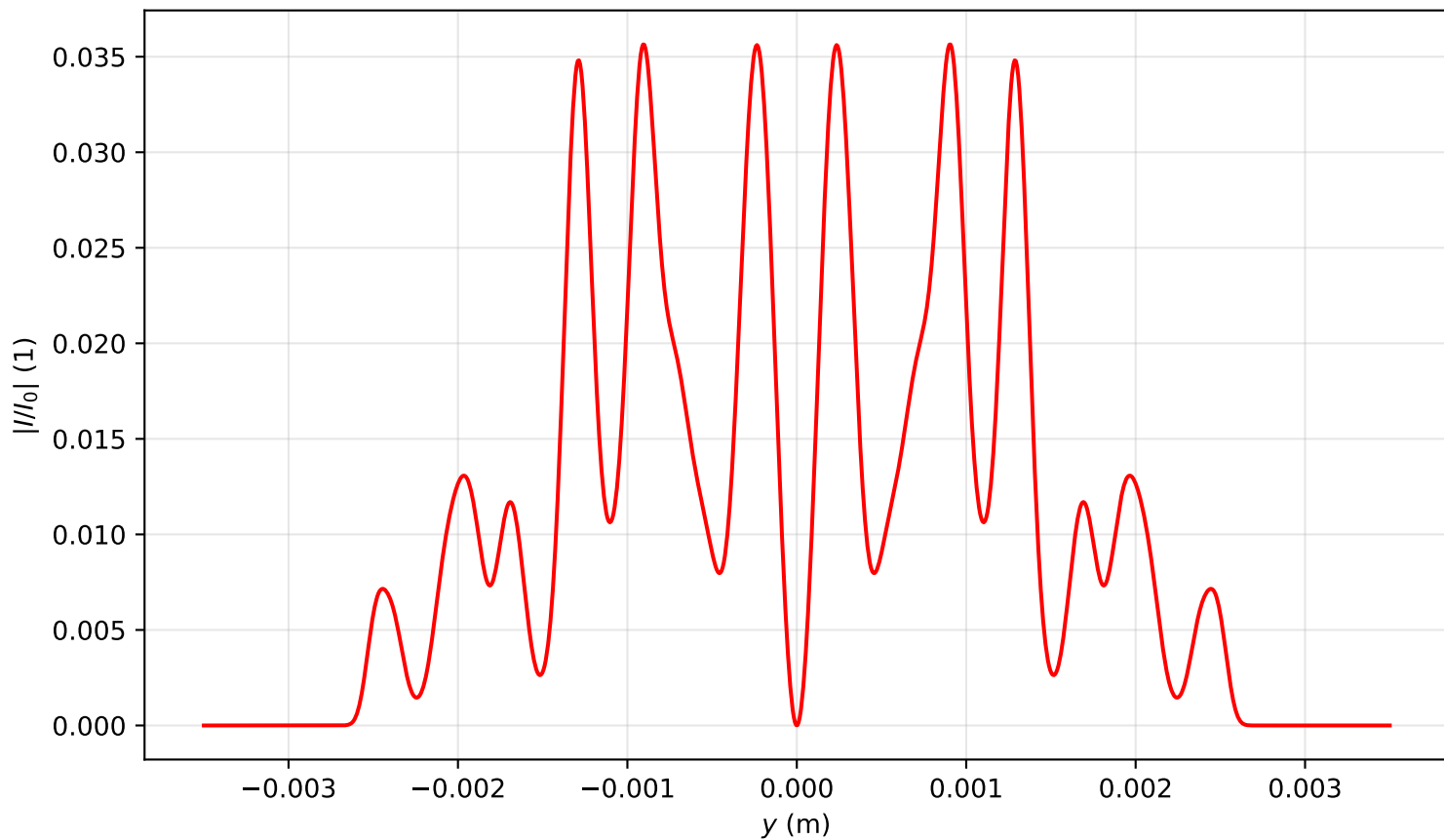
Intensity profile I(x=0, y, z=3.105)/I_0 , P_{in}=8.0P_{cr} , artificial time
